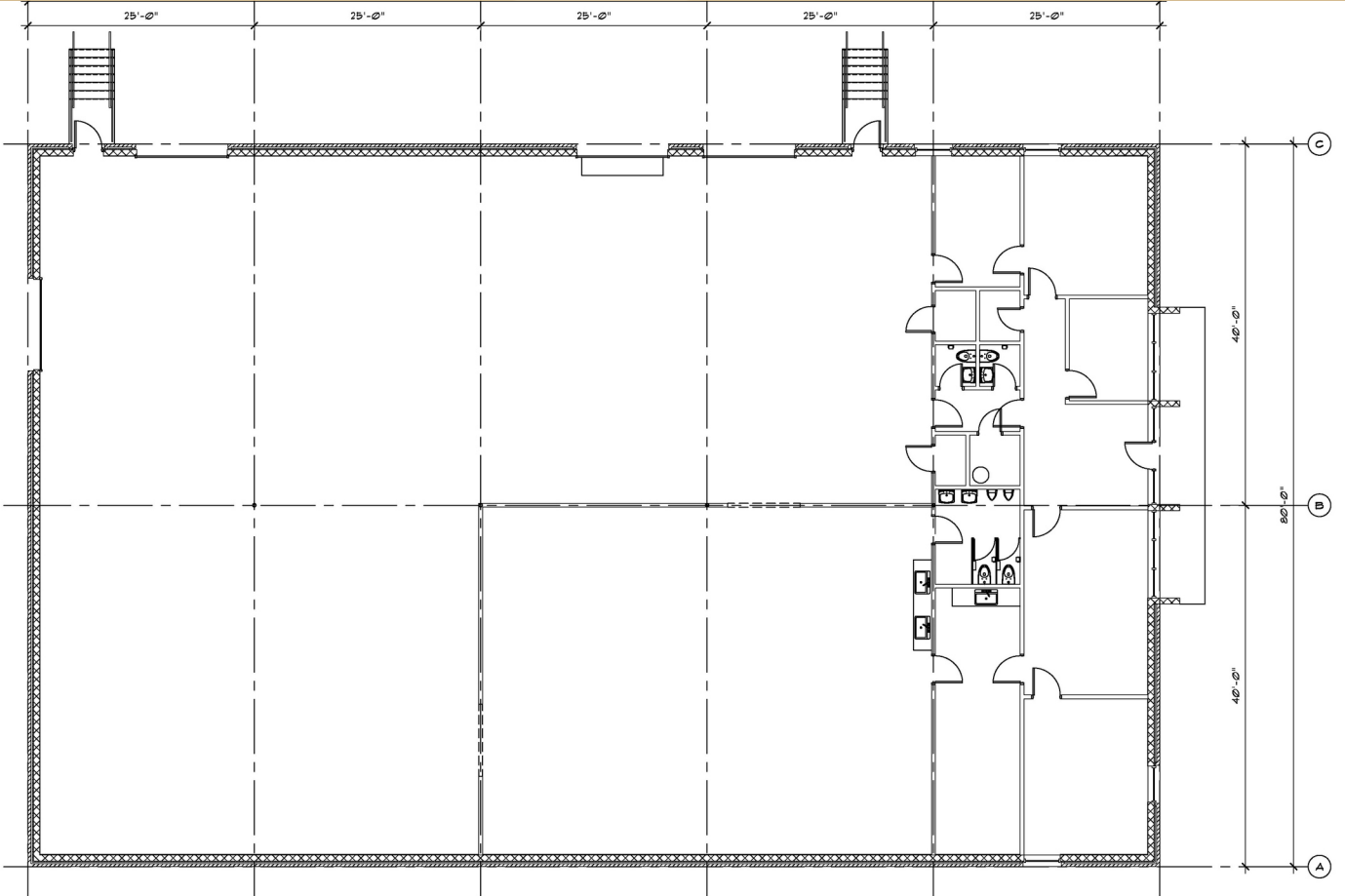
1 BUILDING PLAN
